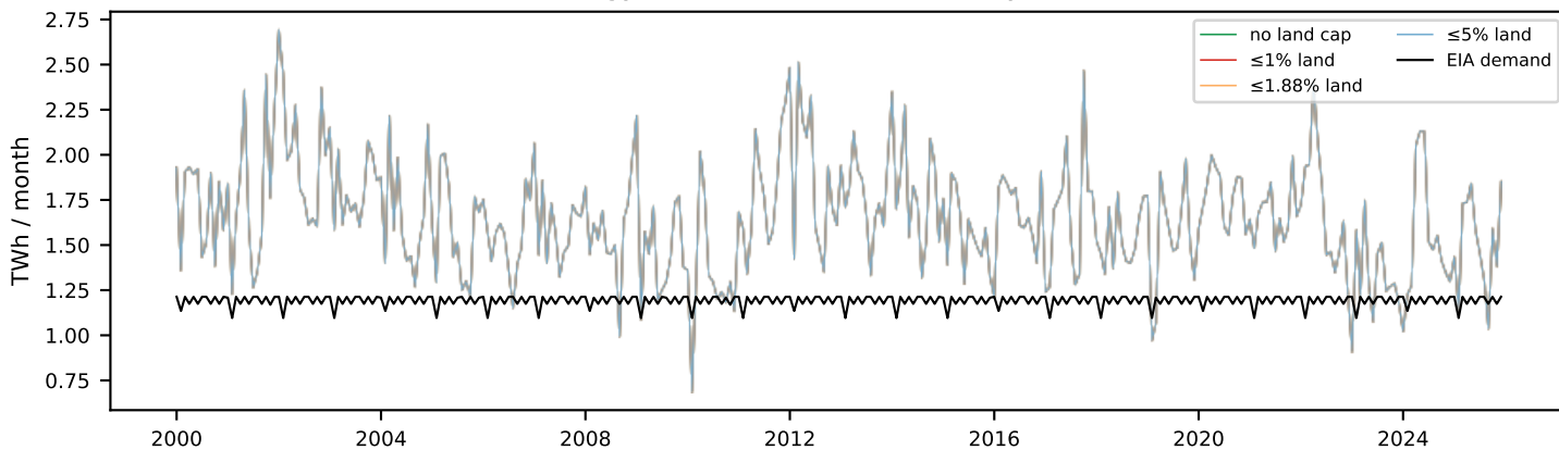
Real energy vs EIA demand (14 TWh/yr, 0.0% land)
