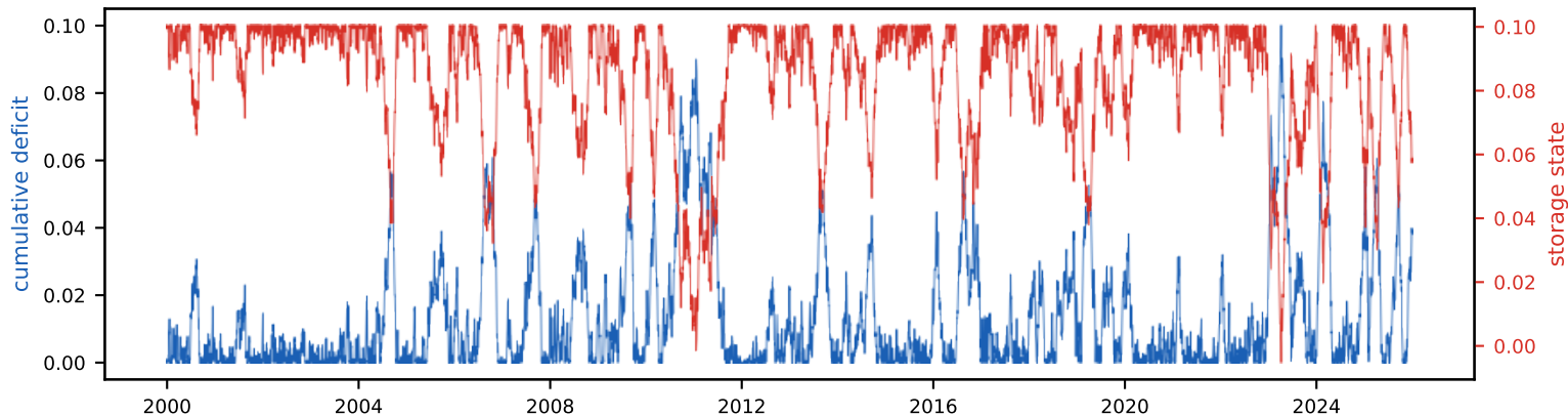
Cumulative deficit & storage state (peak deficit = required storage, S_{tot} =10.0% of annual)
