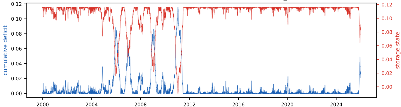
Cumulative deficit & storage state (peak deficit = required storage, S_{\text{tot}} =11.6% of annual)
