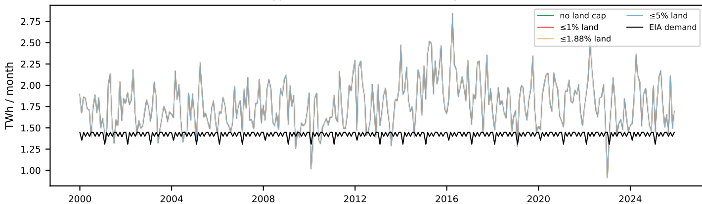
Real energy vs EIA demand (17 TWh/yr, 0.0% land)
