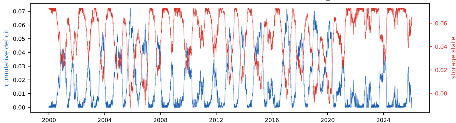
Real energy vs EIA demand (153 TWh/yr, 2.2% land)
