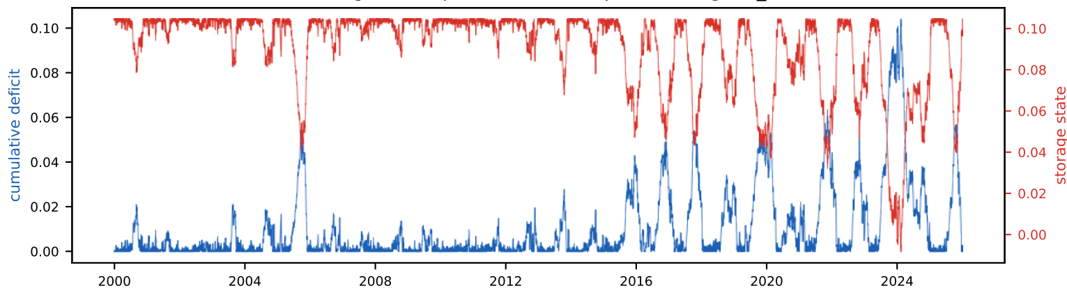
Real energy vs EIA demand (145 TWh/yr, 1.4% land)
