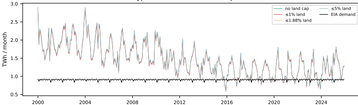
Real energy vs EIA demand (11 TWh/yr, 1.0% land)
