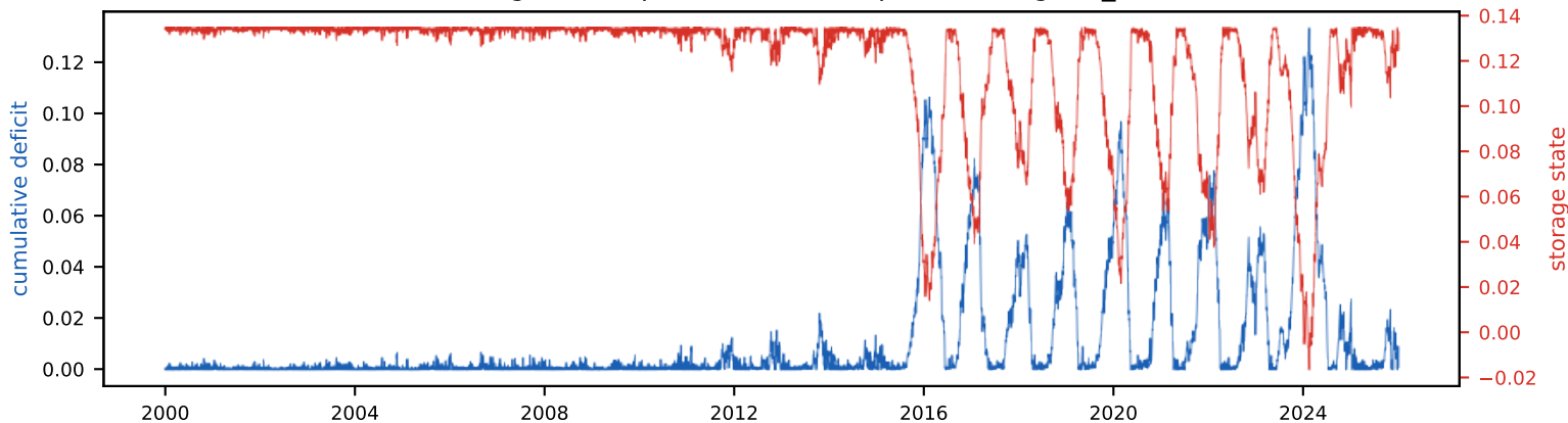
Real energy vs EIA demand (11 TWh/yr, 1.0% land)
