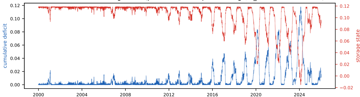
Real energy vs EIA demand (12 TWh/yr, 0.3% land)
