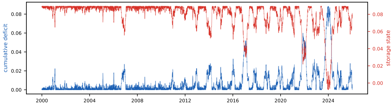
Cumulative deficit & storage state (peak deficit = required storage, S_{\text{tot}} =8.9% of annual)
