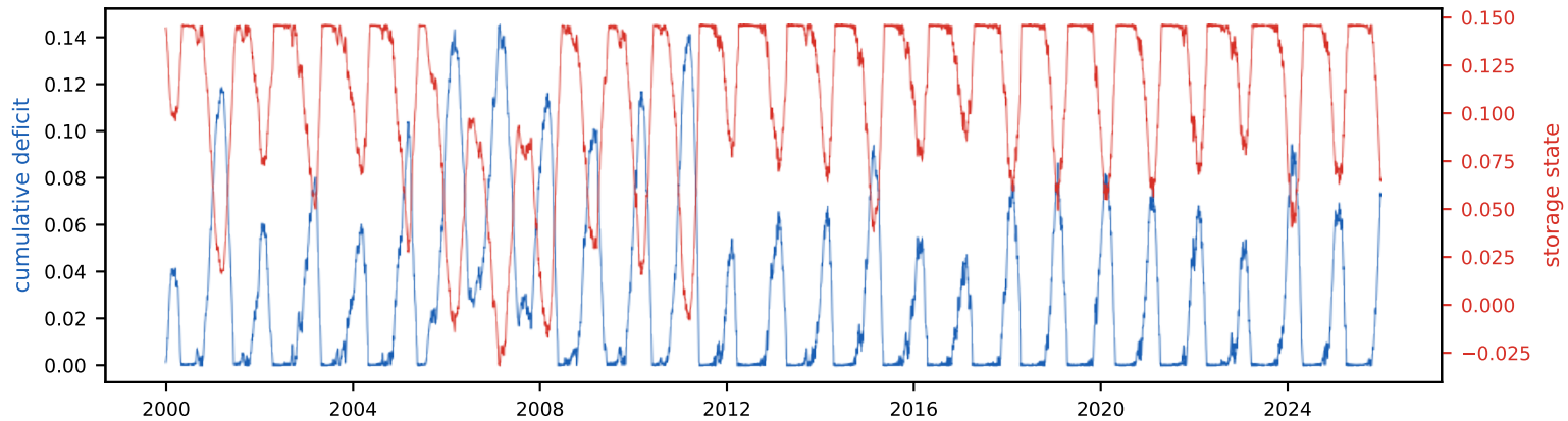
Real energy vs EIA demand (76 TWh/yr, 0.5% land)
