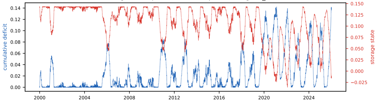
Cumulative deficit & storage state (peak deficit = required storage, S_{\text{tot}} =14.3% of annual)
