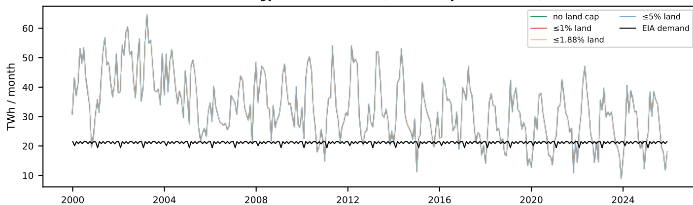
Real energy vs EIA demand (253 TWh/yr, 1.0% land)
