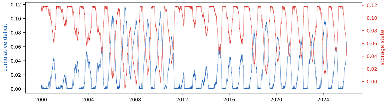
Cumulative deficit & storage state (peak deficit = required storage, S_{\text{tot}} =11.8% of annual)
