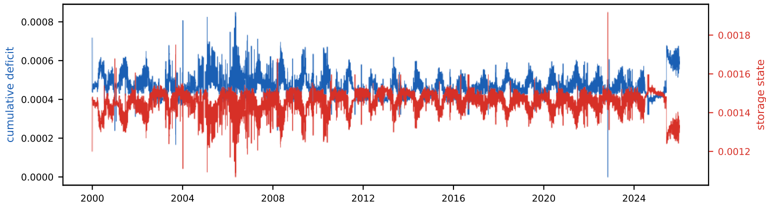
Cumulative deficit & storage state (peak deficit = required storage, S_{\text{tot}} =0.2% of annual)
