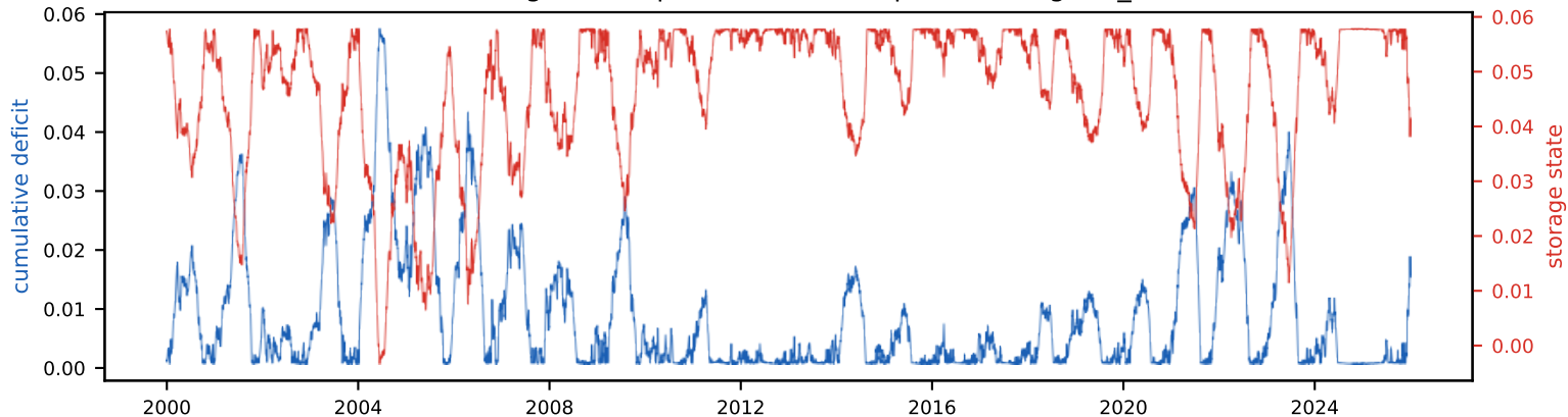
Cumulative deficit & storage state (peak deficit = required storage, S_{\text{tot}} =5.9% of annual)
