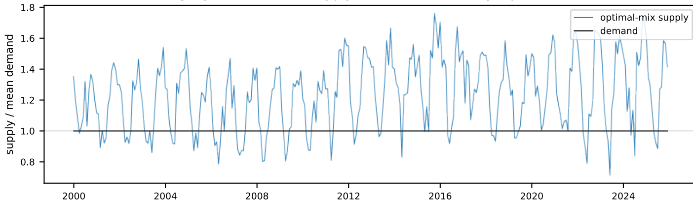
Uruguay — normalized supply vs demand (monthly, optimal mix)
