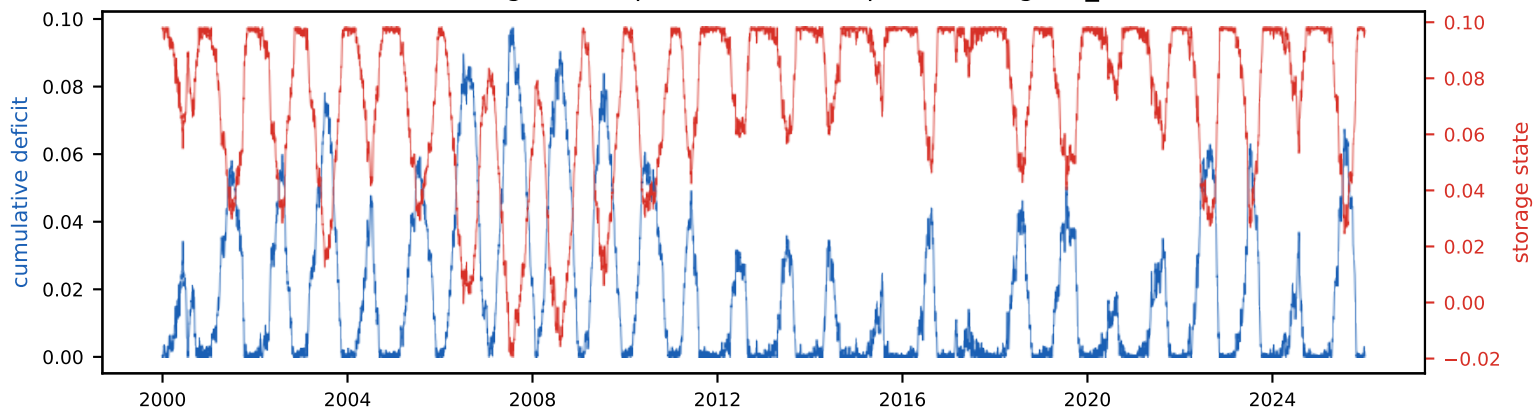
Cumulative deficit & storage state (peak deficit = required storage, S_{\text{tot}} =9.8% of annual)
