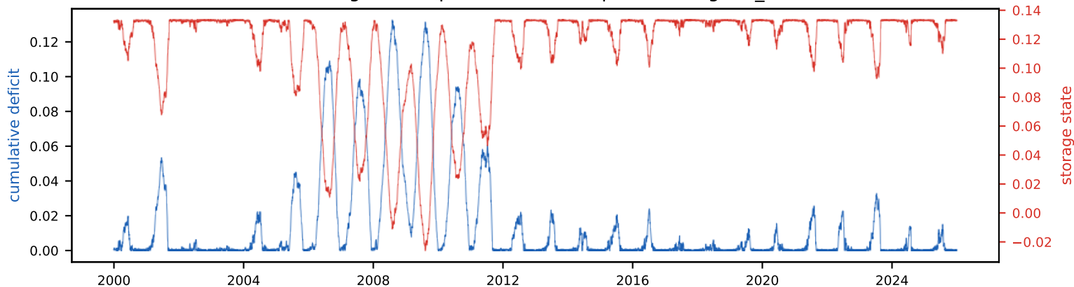
Cumulative deficit & storage state (peak deficit = required storage, S_{\text{tot}} =13.3% of annual)
