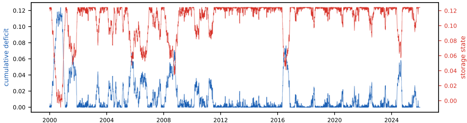
Cumulative deficit & storage state (peak deficit = required storage, S_{\text{tot}} =12.4% of annual)
