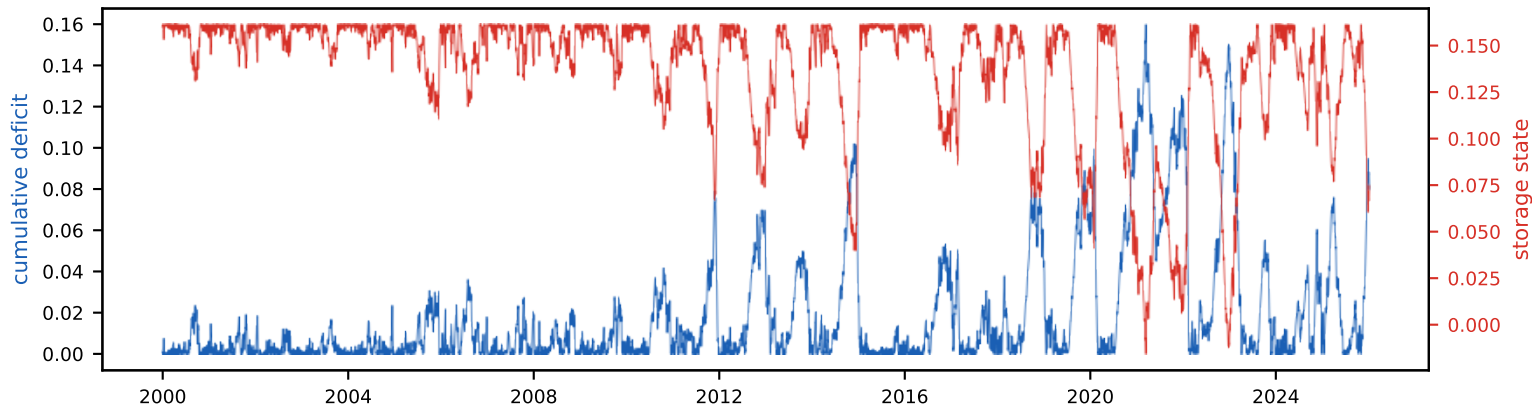
Cumulative deficit & storage state (peak deficit = required storage, S_{\text{tot}} =16.1% of annual)
