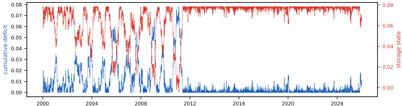
Cumulative deficit & storage state (peak deficit = required storage, S_{\text{tot}} =7.8% of annual)
