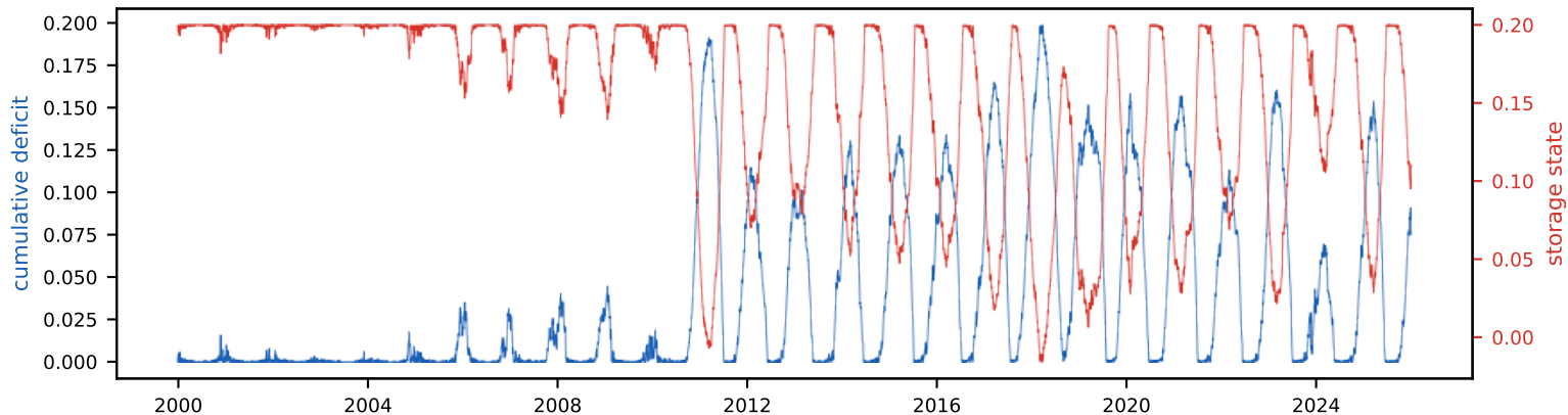
Cumulative deficit & storage state (peak deficit = required storage, S_{\text{tot}} =20.0% of annual)
