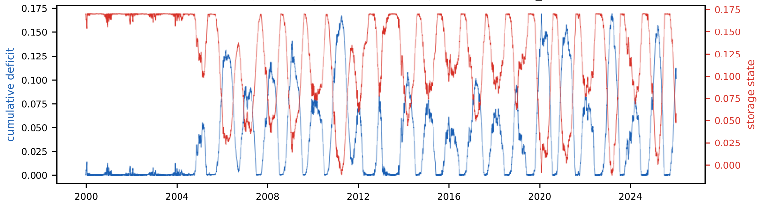
Cumulative deficit & storage state (peak deficit = required storage, S_{tot} =17.0% of annual)
