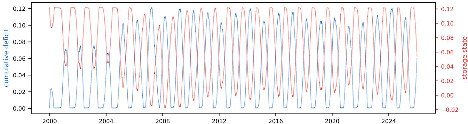
Cumulative deficit & storage state (peak deficit = required storage, S_{\text{tot}} =12.2% of annual)
