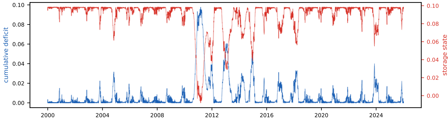
Cumulative deficit & storage state (peak deficit = required storage, S_{tot} =9.8% of annual)
