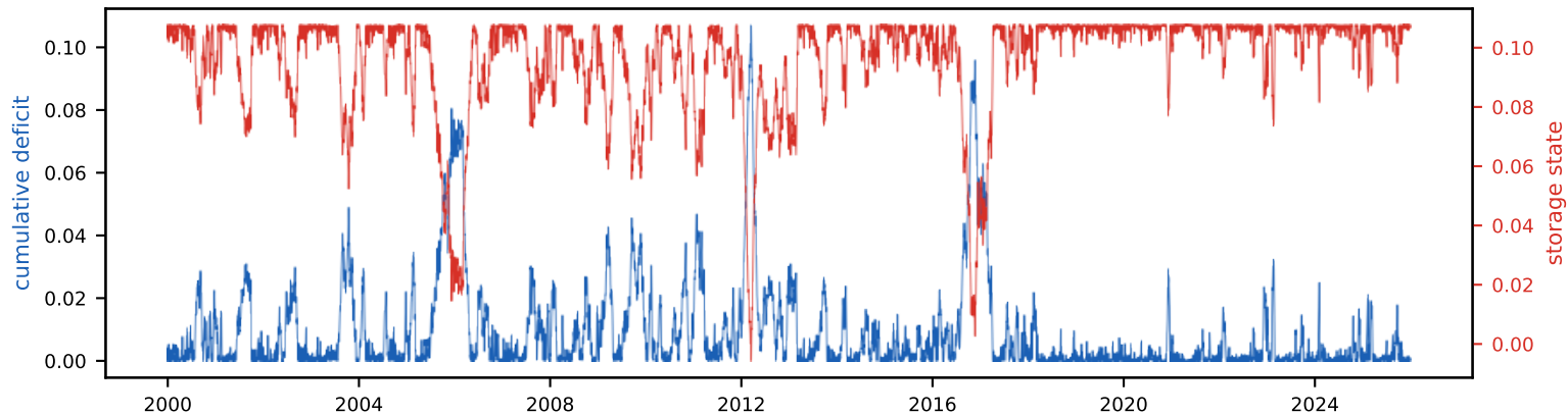
Cumulative deficit & storage state (peak deficit = required storage, S_{\text{tot}} =10.8% of annual)
