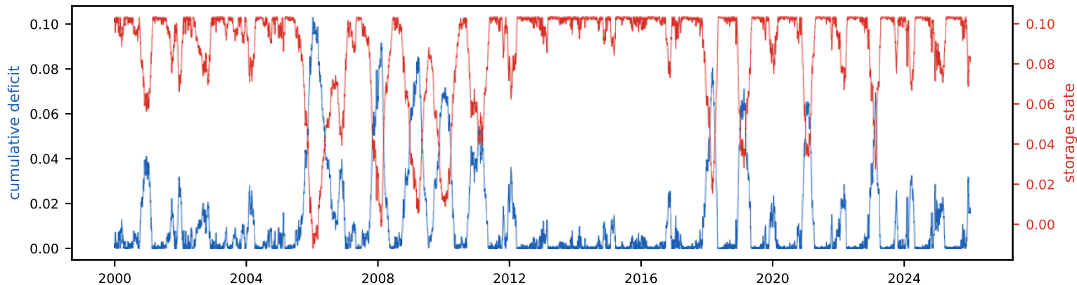
Cumulative deficit & storage state (peak deficit = required storage, S_{\text{tot}} =10.3% of annual)
