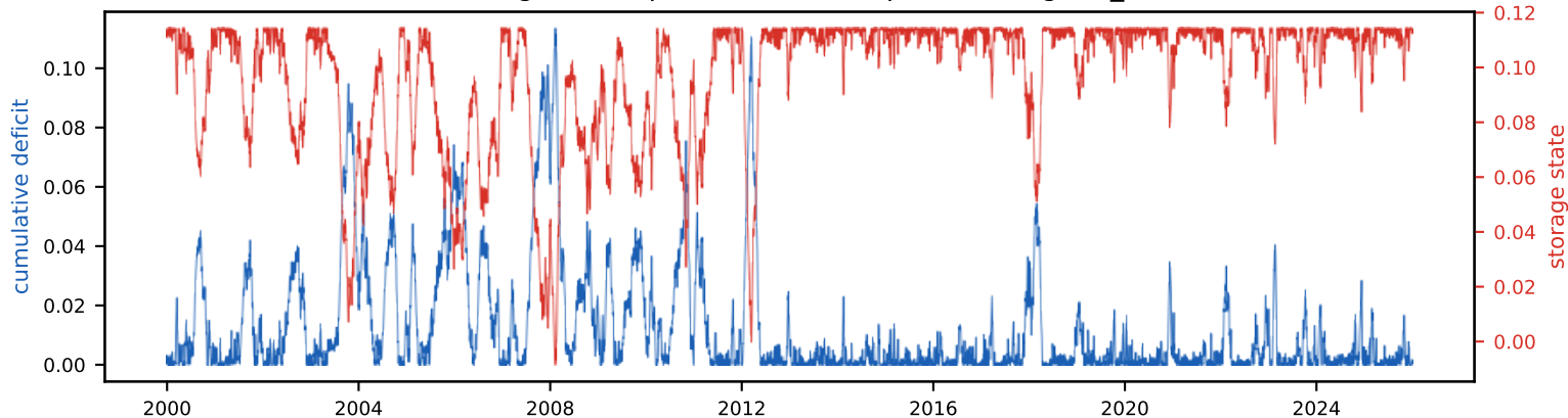
Cumulative deficit & storage state (peak deficit = required storage, S_{\text{tot}} =11.4% of annual)
