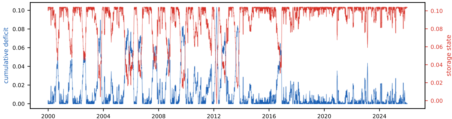
Cumulative deficit & storage state (peak deficit = required storage, S_{\text{tot}} =10.4% of annual)
