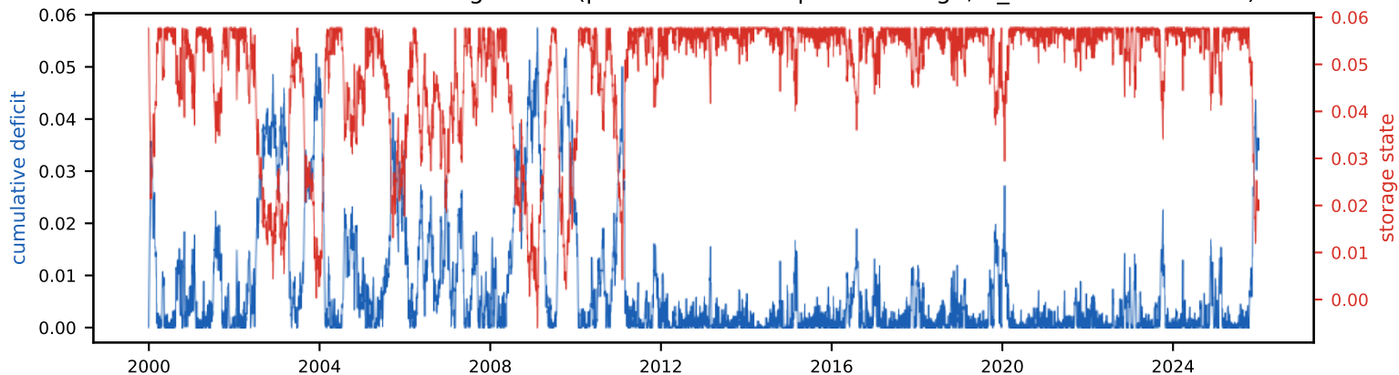
Cumulative deficit & storage state (peak deficit = required storage, S_{\text{tot}} =5.8% of annual)
