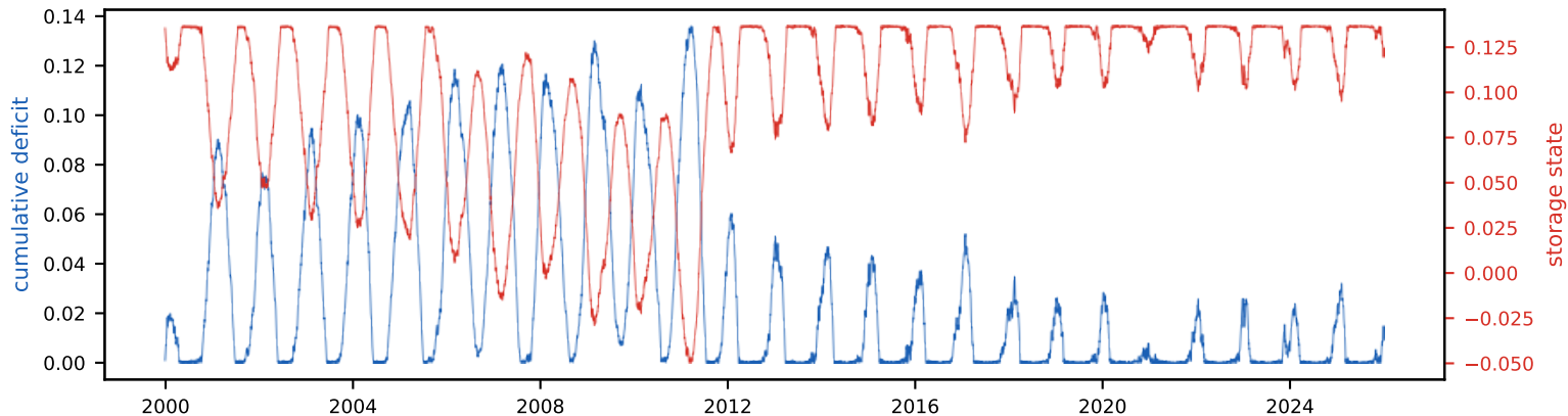
Cumulative deficit & storage state (peak deficit = required storage, S_{\text{tot}} =13.6% of annual)
