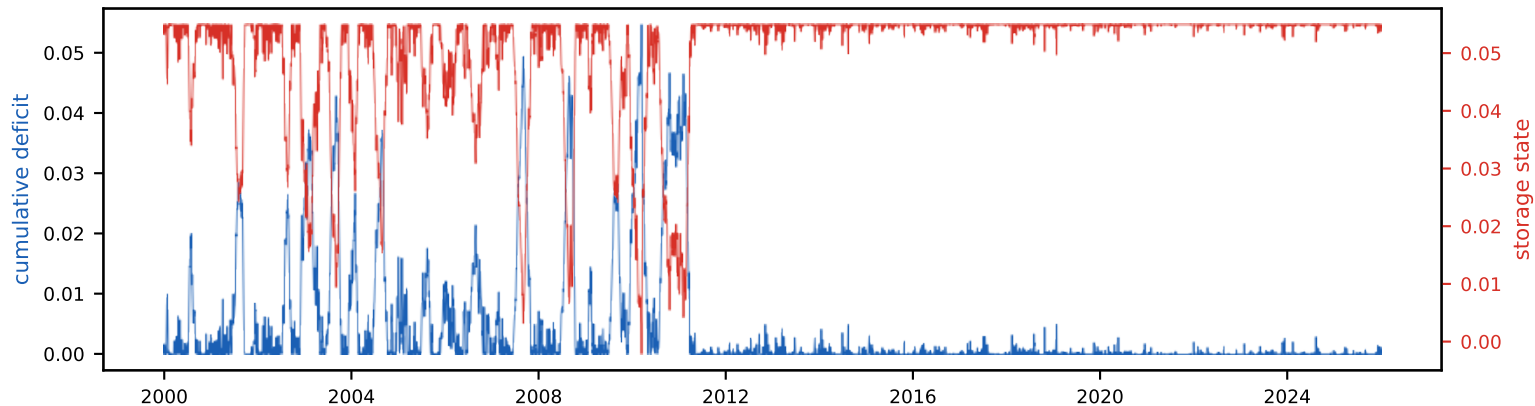
Cumulative deficit & storage state (peak deficit = required storage, S_{tot}=5.5\% of annual)
