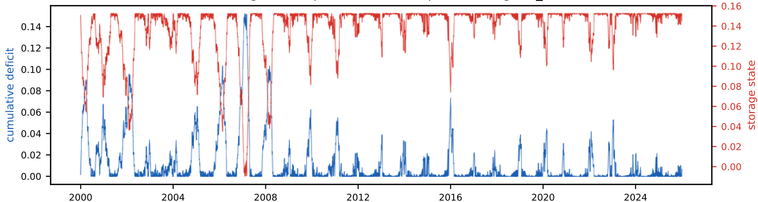
Cumulative deficit & storage state (peak deficit = required storage, S_{\text{tot}} =15.2% of annual)
