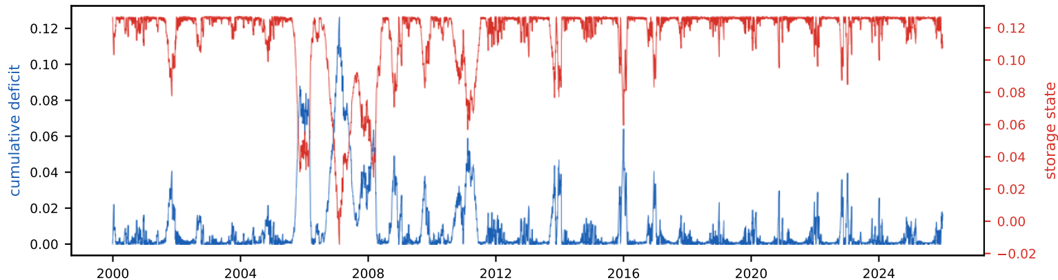
Cumulative deficit & storage state (peak deficit = required storage, S_{\text{tot}} =12.7% of annual)
