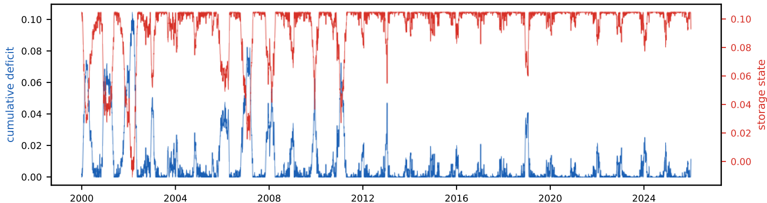
Cumulative deficit & storage state (peak deficit = required storage, S_{\text{tot}} =10.5% of annual)
