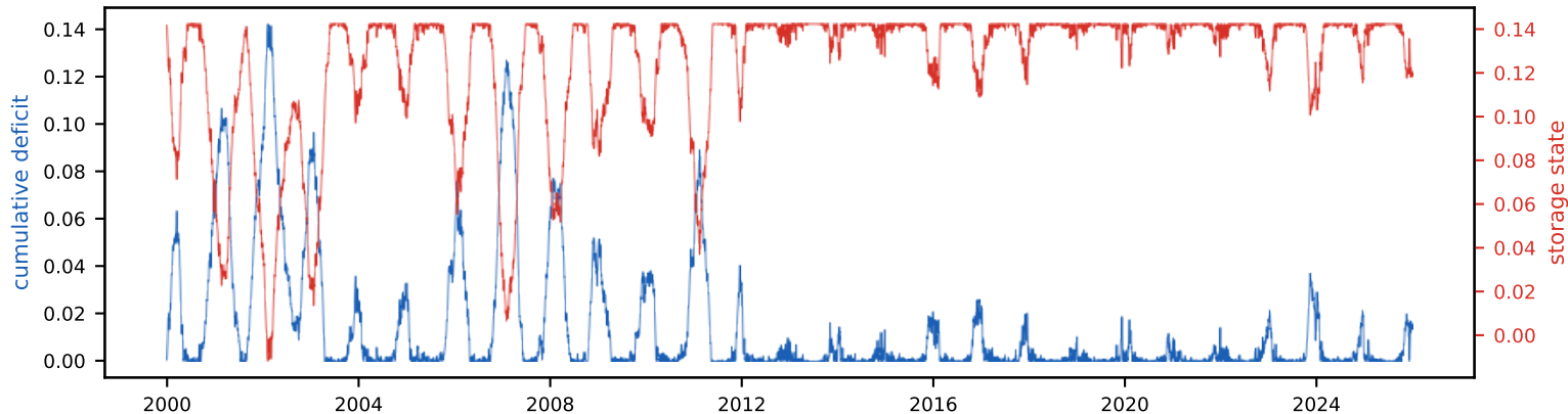
Cumulative deficit & storage state (peak deficit = required storage, S_{\text{tot}} =14.2% of annual)
