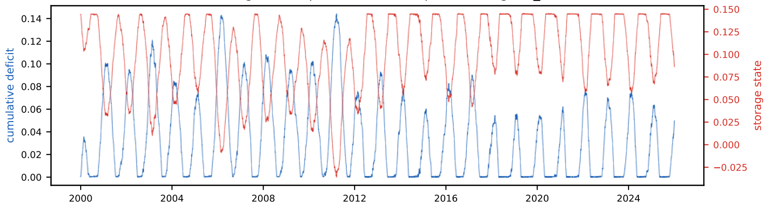
Cumulative deficit & storage state (peak deficit = required storage, S_{\text{tot}} =14.5% of annual)
