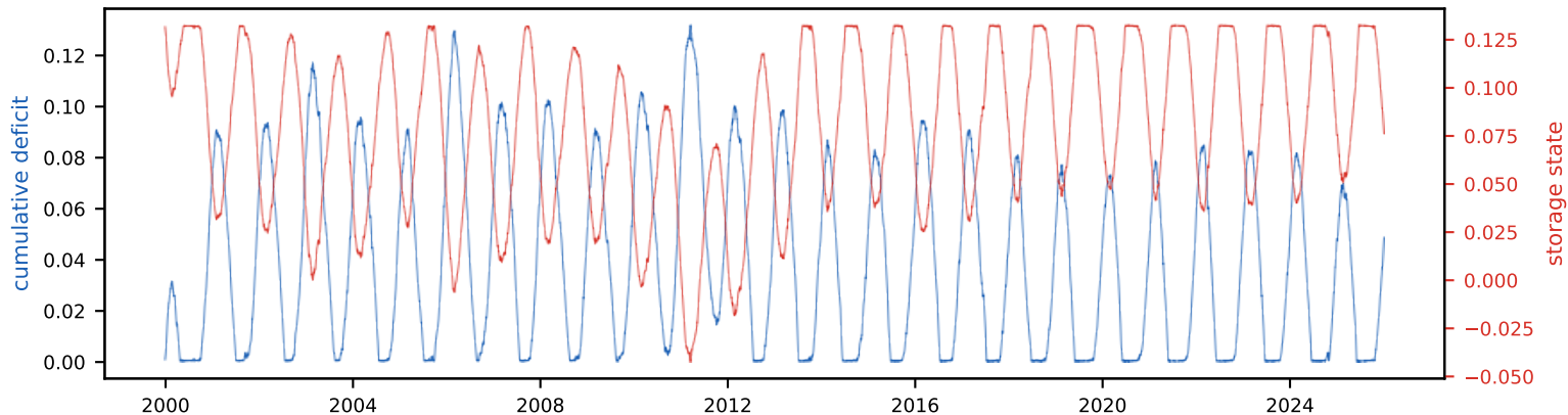
Cumulative deficit & storage state (peak deficit = required storage, S_{\text{tot}} =13.3% of annual)
