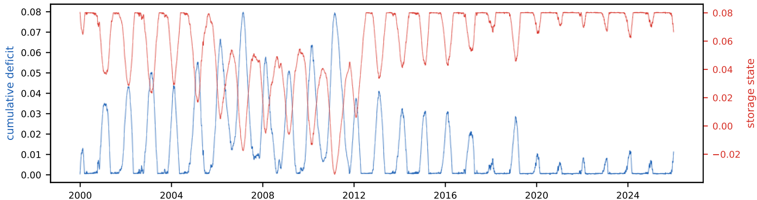
Cumulative deficit & storage state (peak deficit = required storage, S_{tot}=8.1\% of annual)
