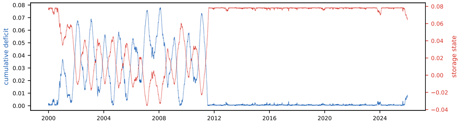
Cumulative deficit & storage state (peak deficit = required storage, S_{\text{tot}} =7.9% of annual)
