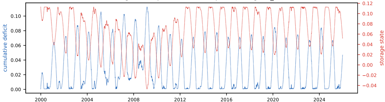
Cumulative deficit & storage state (peak deficit = required storage, S_{\text{tot}} =11.3% of annual)
