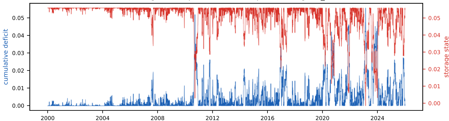
Real energy vs EIA demand (6 TWh/yr, 0.0% land)
