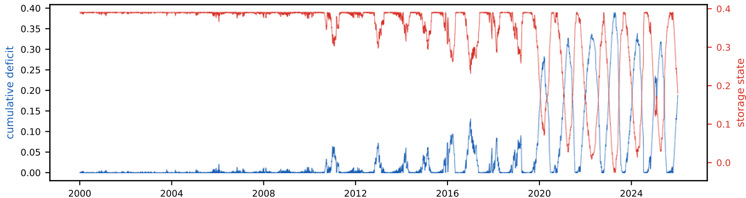
Cumulative deficit & storage state (peak deficit = required storage, S_{\text{tot}} =39.0% of annual)
