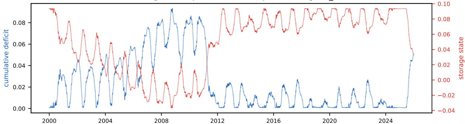
Cumulative deficit & storage state (peak deficit = required storage, S_{\text{tot}} =9.4% of annual)
