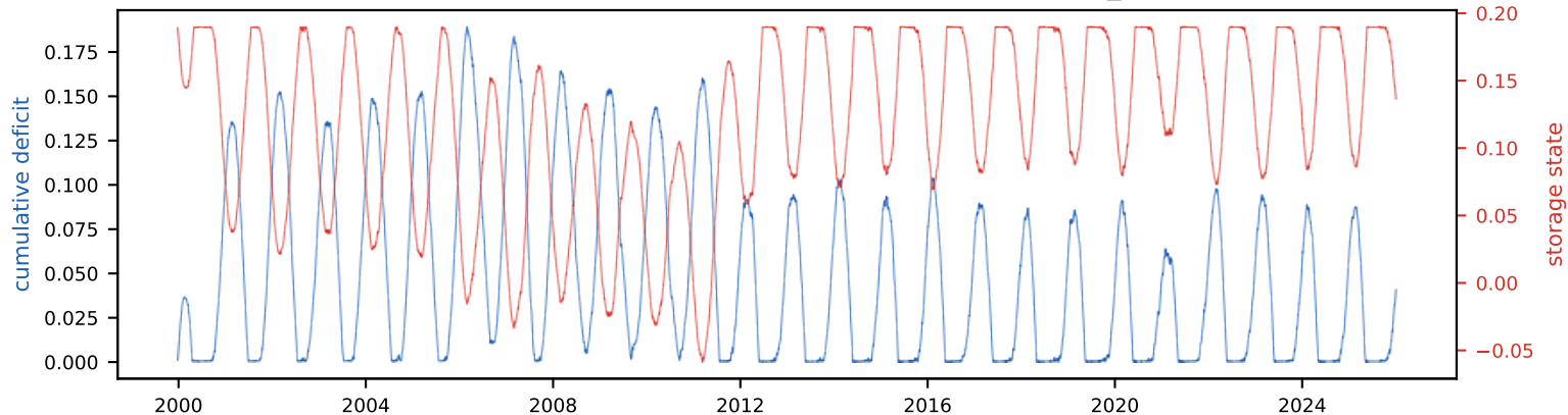
Cumulative deficit & storage state (peak deficit = required storage, S_{\text{tot}} =19.0% of annual)
