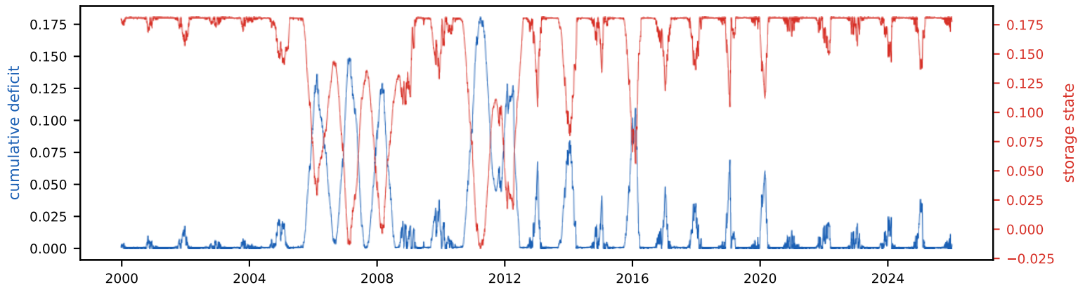
Cumulative deficit & storage state (peak deficit = required storage, S_{\text{tot}} =18.1% of annual)
