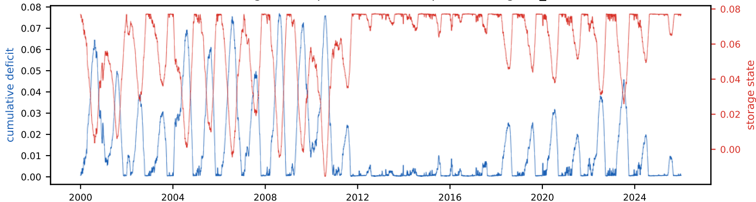
Cumulative deficit & storage state (peak deficit = required storage, S_{\text{tot}} =7.8% of annual)
