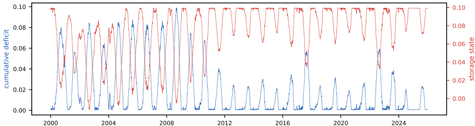
Cumulative deficit & storage state (peak deficit = required storage, S_{\text{tot}} =10.0% of annual)
