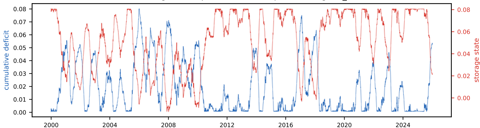
Cumulative deficit & storage state (peak deficit = required storage, S_{\text{tot}} =8.1% of annual)
