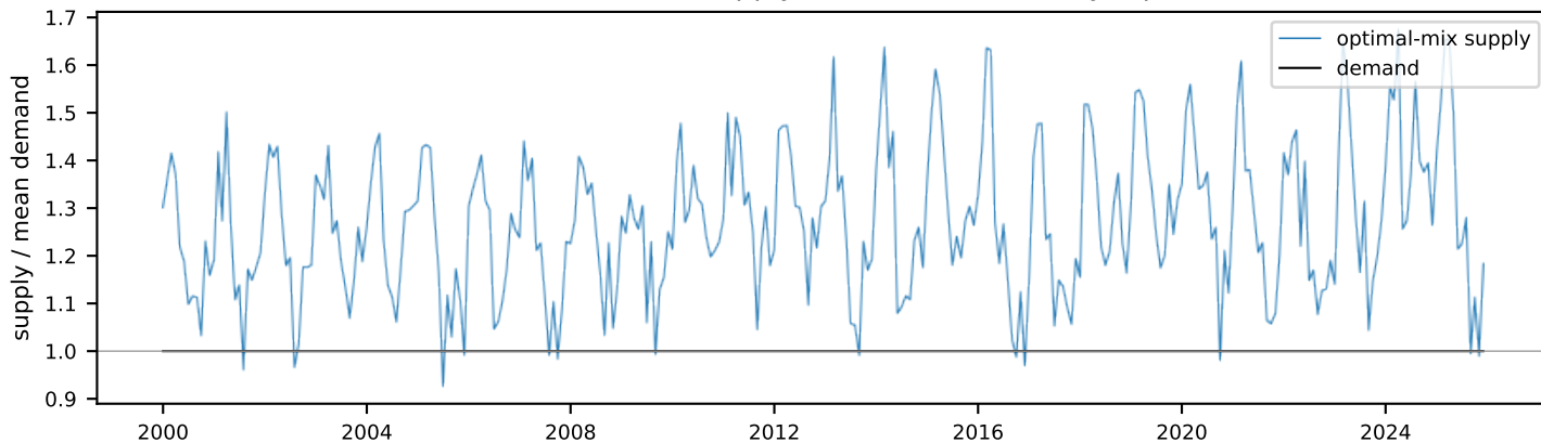
Cambodia — normalized supply vs demand (monthly, optimal mix)
