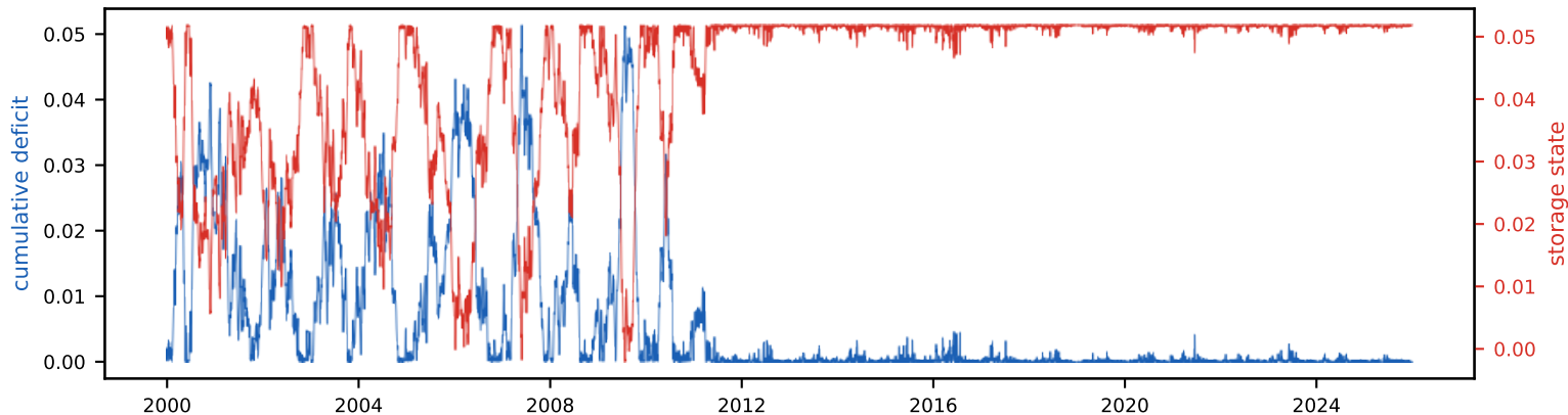
Cumulative deficit & storage state (peak deficit = required storage, S_{\text{tot}} =5.2% of annual)
