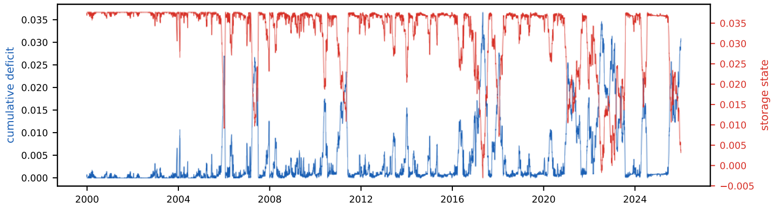
Cumulative deficit & storage state (peak deficit = required storage, S_{\text{tot}} =3.8% of annual)
